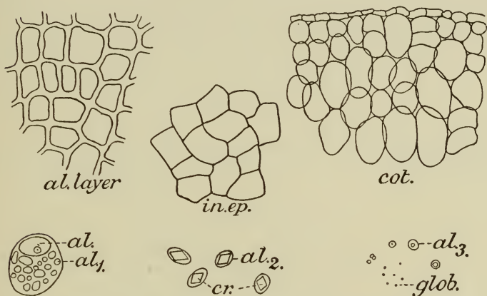
FIG. 130.—Almond. al. layer , aleurone layer in surface view; cot. , cotyledon, in transverse section; in. ep. , inner epidermis of seed coat; al. , large aleurone grain; al 1 , small aleurone grain. All \times 240 . al 2 , al 3 , small aleurone grains; cr. , crystalloids; glob. , globoids. \times 480
